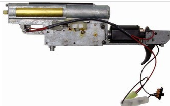
AB-5873T-GB AE-5873-T Metal Gearbox w/Motor & Metal Bushing
